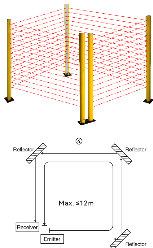
4. Four-sided Regional Safety Protection
