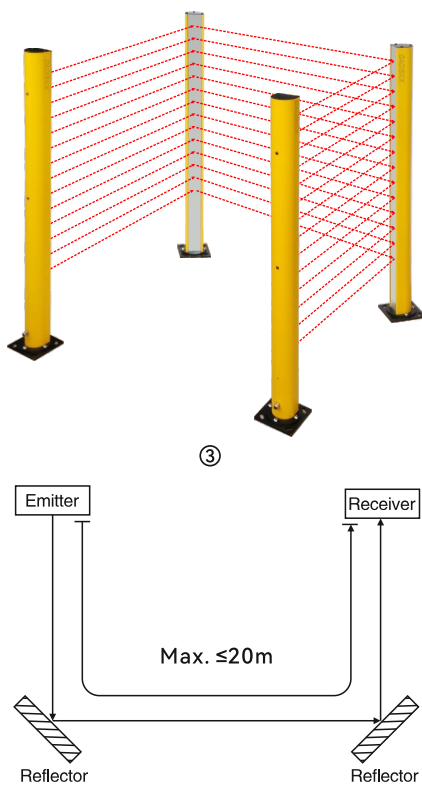
3. Three-sided Regional Safety Protection
