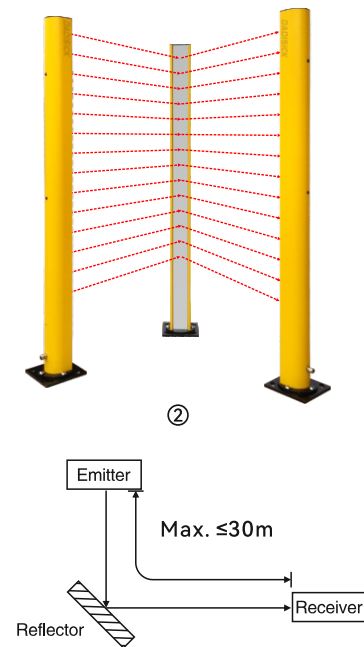
2. Two-sided Regional Safety Protection
