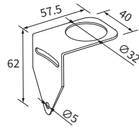
O50/O70 brackets
