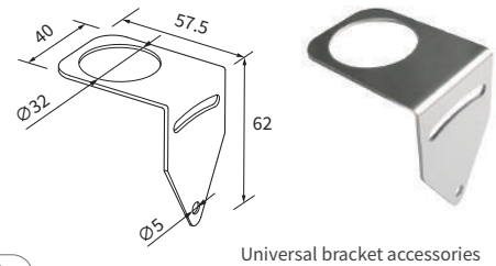
Universal bracket accessories
